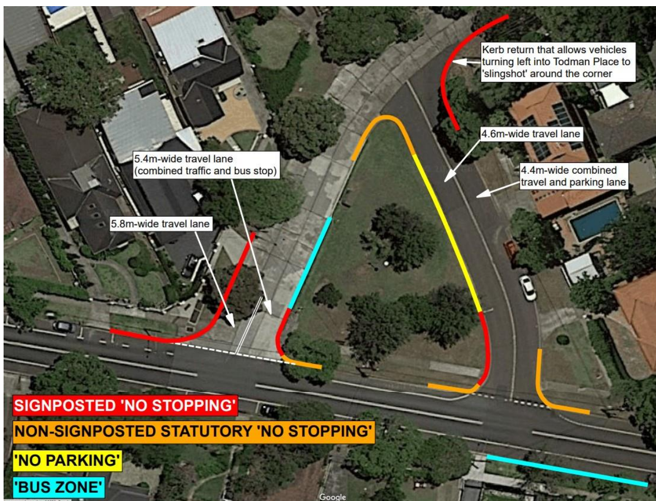
Figure 1 – existing signs and line marking around Todman Reserve
