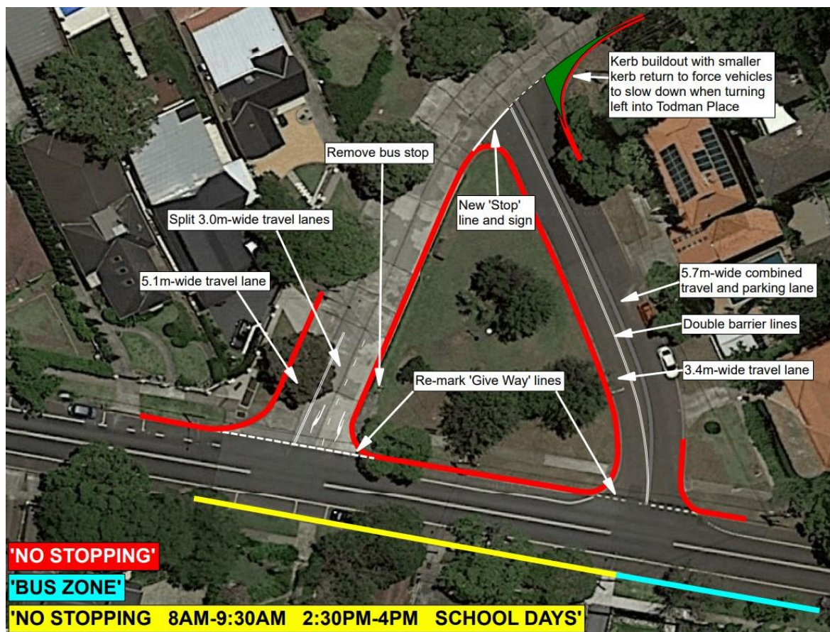
Figure 2 – final signs, line marking, and kerb buildout around Todman Reserve
