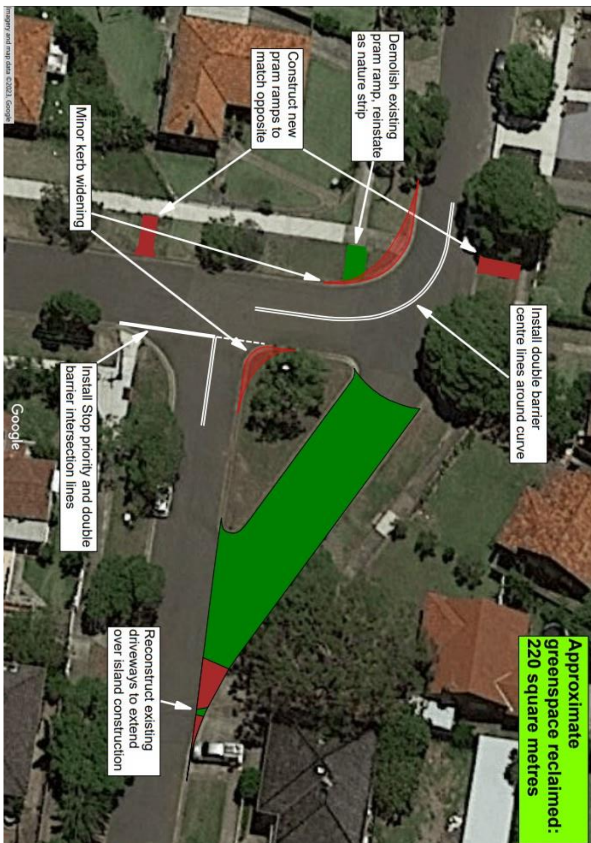
Figure 1 – proposed full road closure of Mintaro Avenue and supporting changes
