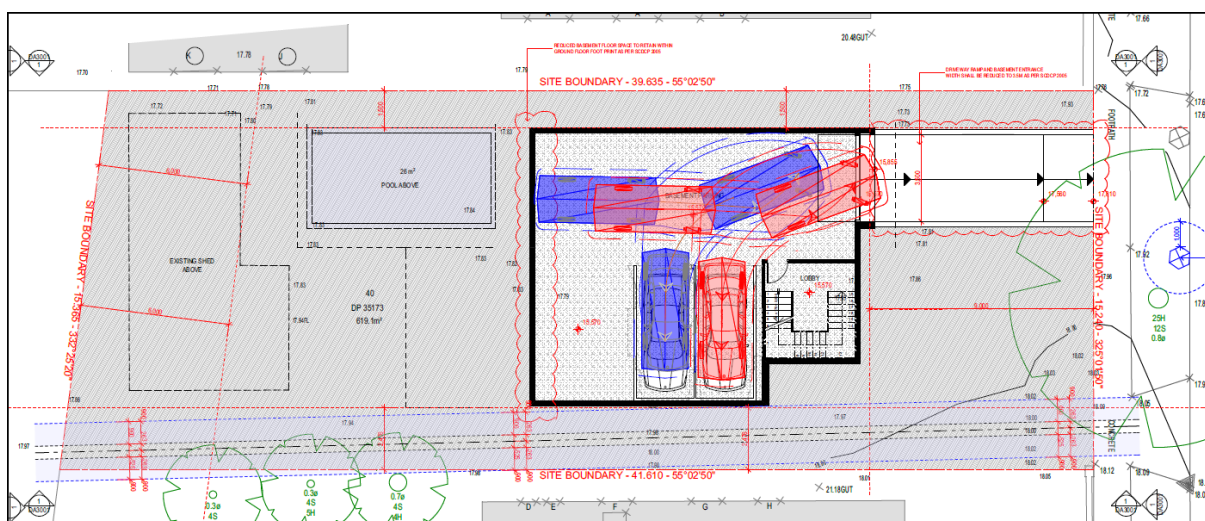
Figure 2: Proposed basement plan
