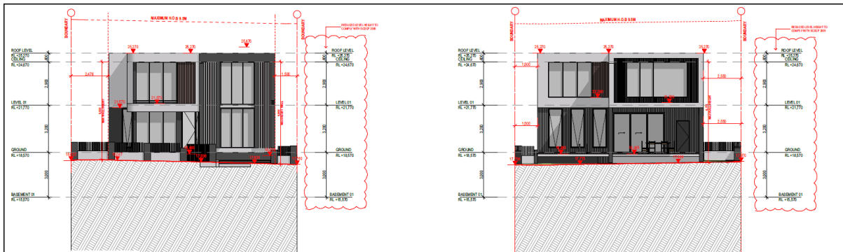
Figure 7: Proposed east and west elevations (left to right)
